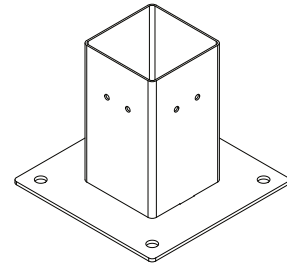
BASE PILAR
